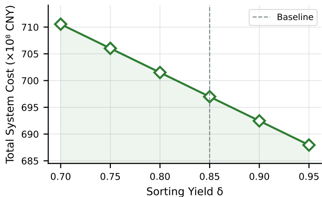
(c) System Cost vs. Sorting Efficiency
