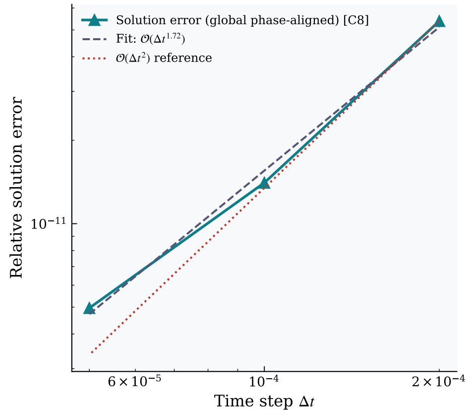
(a) Temporal convergence (BAB Strang splitting, 2nd order)
