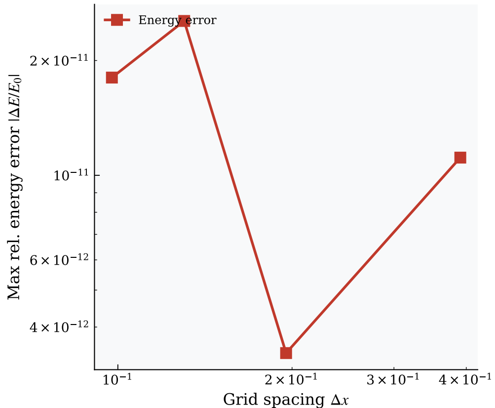
(b) Spatial convergence (pseudo-spectral)
