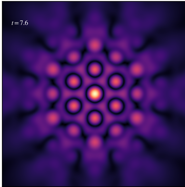
(b) fusion ( \nu=1.0 )
