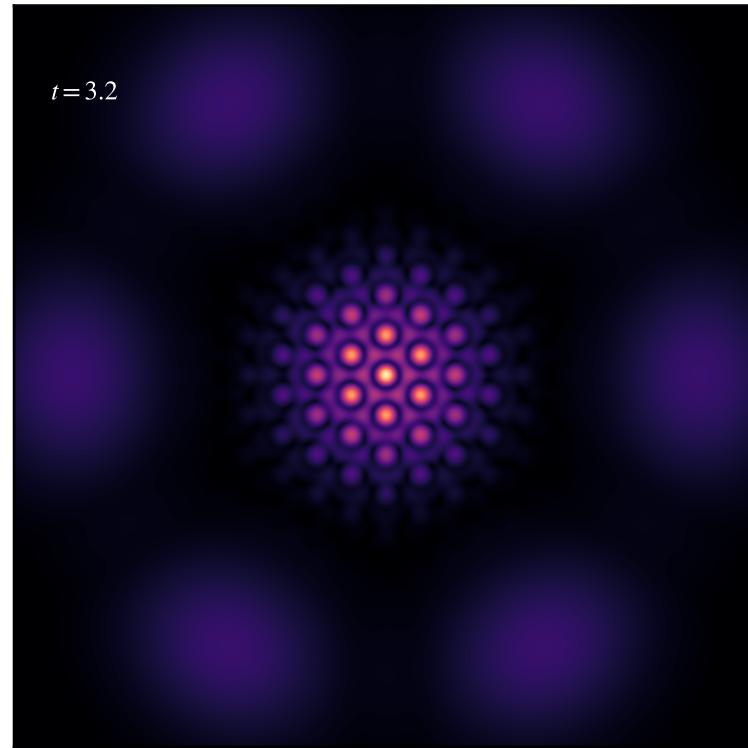
(c) collapse ( \nu=3.0 )
