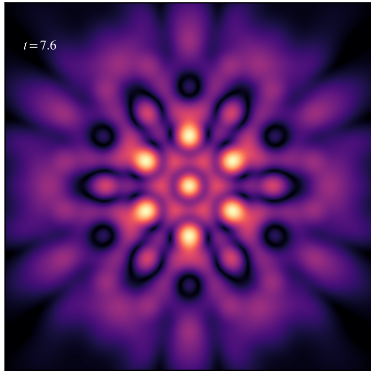
(a) fragmentation ( \nu=0.5 )
