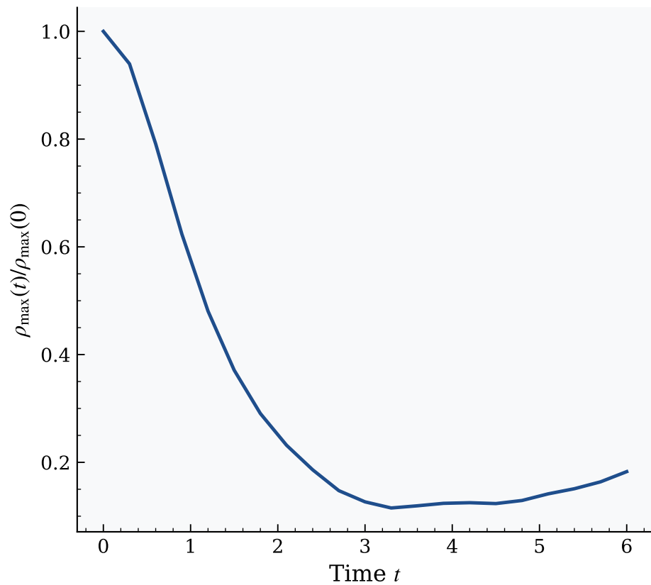
(a) Single ring density peak
