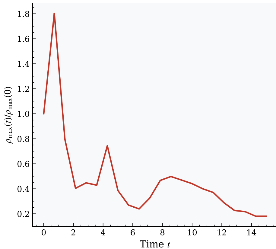
(b) Collision density peak
