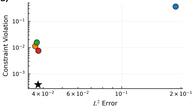
(c) Nonlinear Schrödinger
