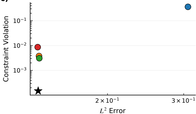
(c) Nonlinear Schrödinger
