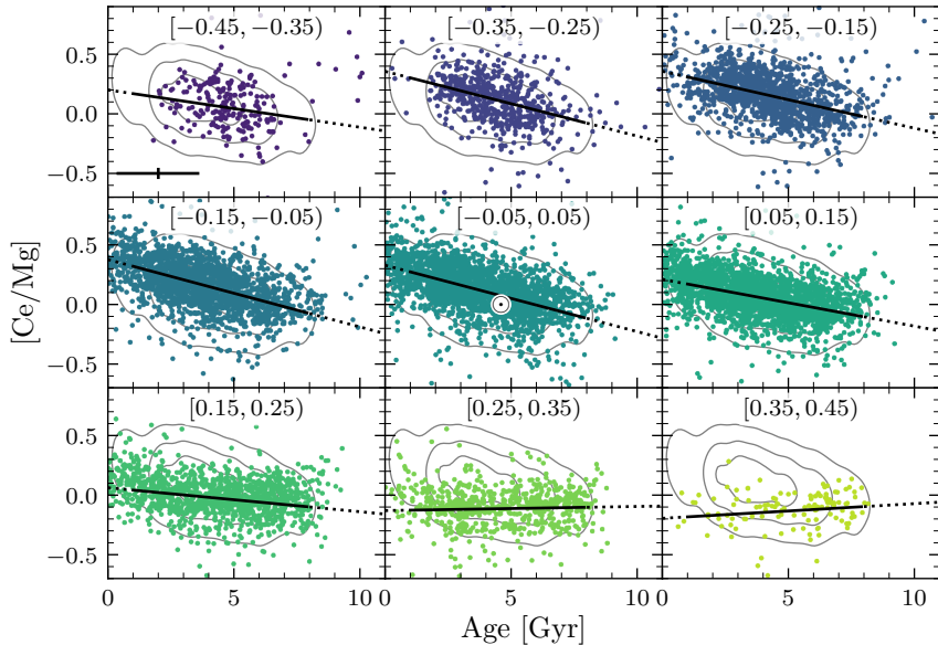
Bins in [\text{Fe}/\text{H}] (High-Ia stars only)
