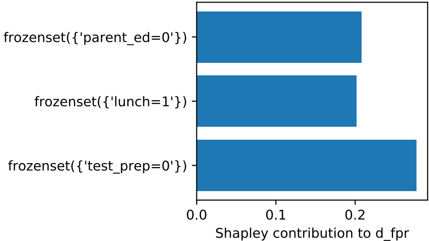
students_figure_3: Approximate Shapley contributions for most FPR-divergent pattern
