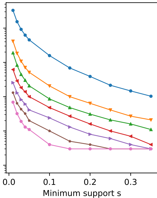
adult
