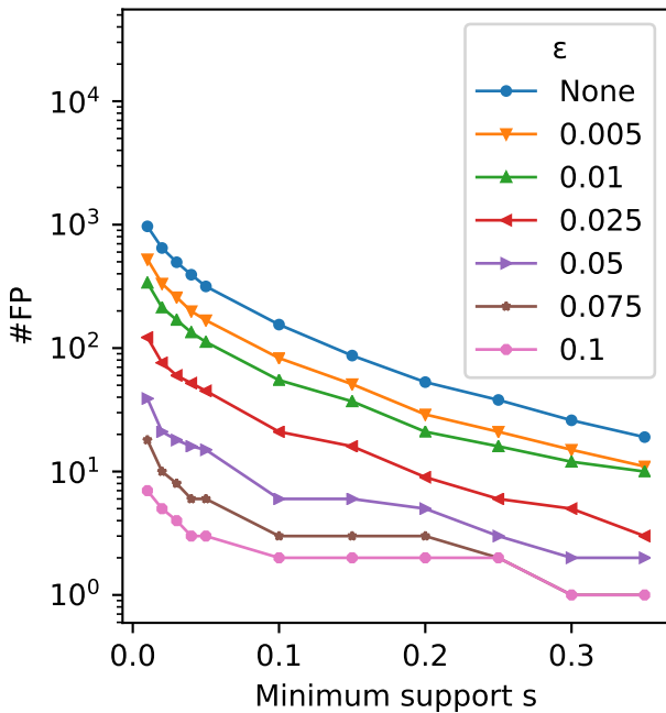
COMPAS
