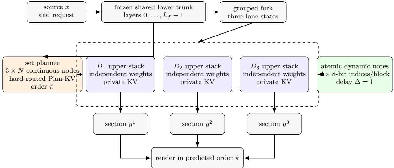
Figure 1: The Parallel Decoder Transformer. Solid arrows carry token states; dashed arrows carry persistent plan memory or block-delayed latent messages. The physical decoder stacks advance together but do not share upper weights or KV state.
