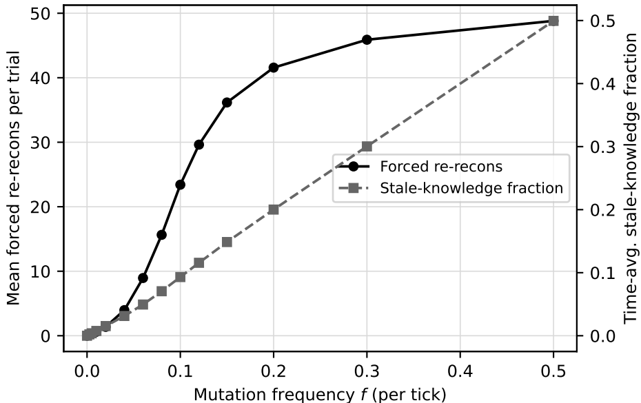
Attacker uncertainty vs. mutation frequency
