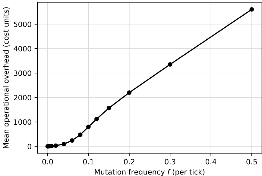
Operational overhead vs. mutation frequency
