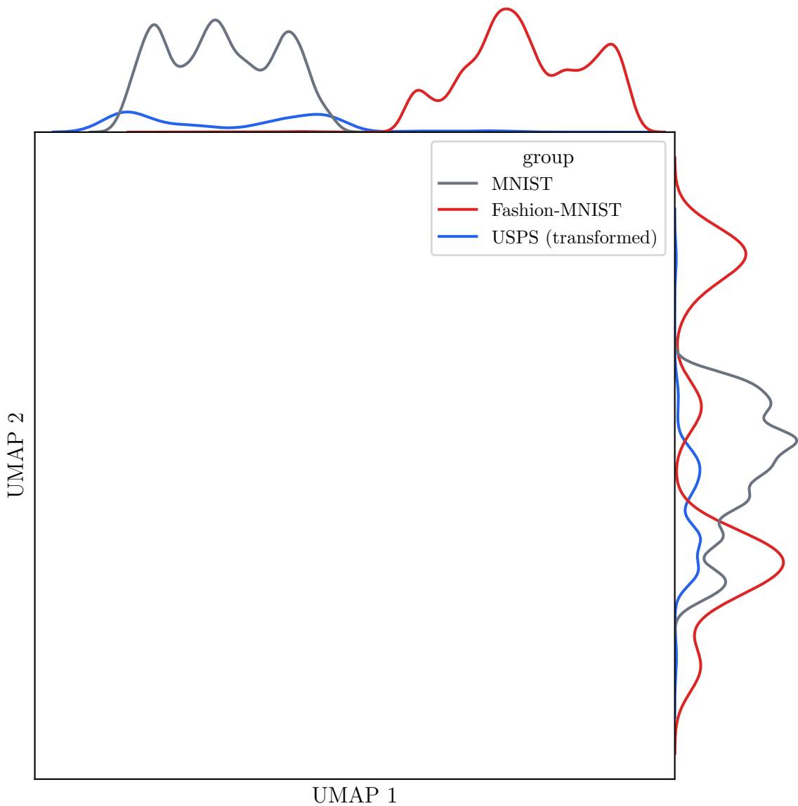
INCEPTION UMAP Marginal Density: MNIST, Fashion-MNIST, USPS
