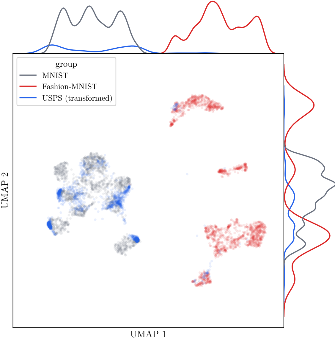
INCEPTION UMAP Marginal Density + Points: MNIST, Fashion-MNIST, USPS
