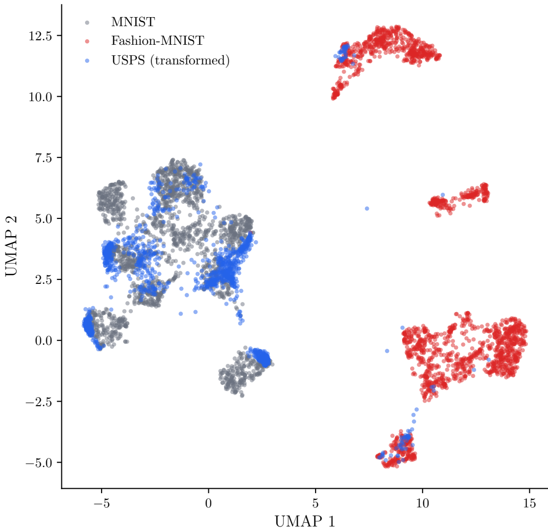
INCEPTION UMAP: MNIST, Fashion-MNIST, USPS
