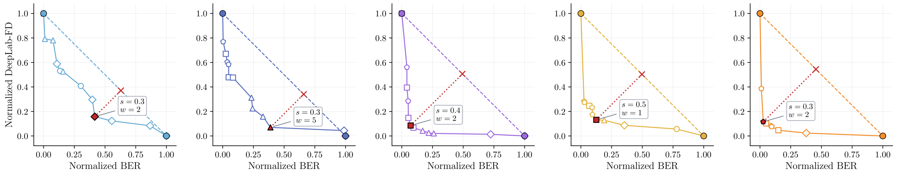
Knee Selection
