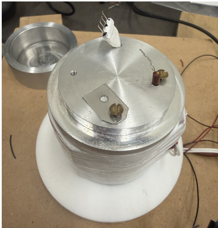
Figure 7: The sample chamber with its metal cup cover removed, showing the sample clip, pins for connecting the PCB, and cable to the PID temperature controller.
