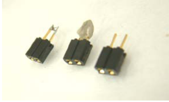
Figure 9: An empty two-pin connector (right), a mounted BaTiO 3 sample (center), and a 100 pF test capacitor soldered to the connector (left).
