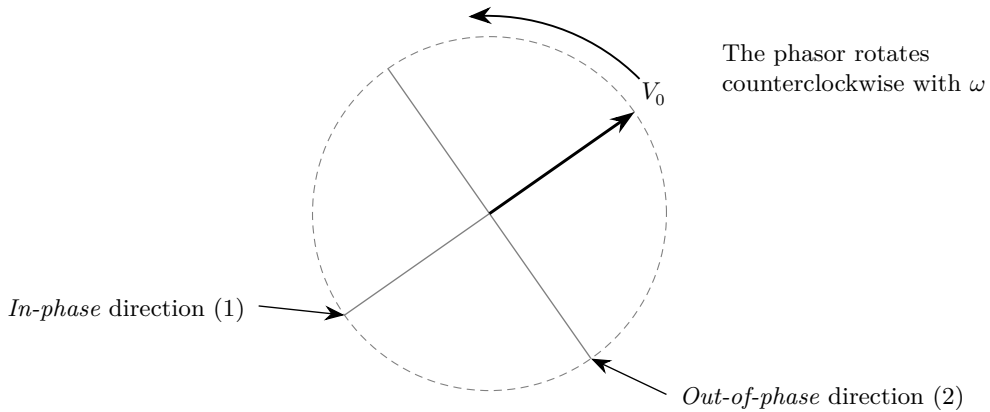
Figure 13: The in-phase and out-of-phase reference directions, defined relative to the source voltage V_0 .
