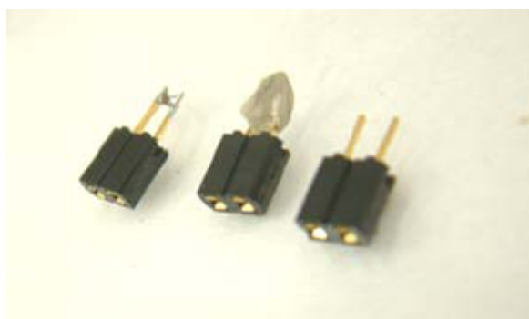
Figure 9: An empty two-pin connector (right), a mounted \text{BaTiO}_3 sample (center), and a 100 pF test capacitor soldered to the connector (left).
