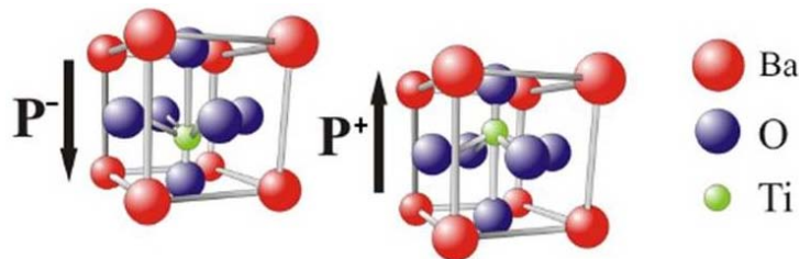
Fig. 8. Unit cells of BaTiO 3 with (green) Ti ion in two off-center positions: with p pointing up (called p^+ here) and with p pointing down (called p^- here). Below T_C , dipole moments p^+ and p^- spontaneously appear without an external field. If there is an electric field E , for example, pointing up, than p^+ will have lower energy than p^- .
