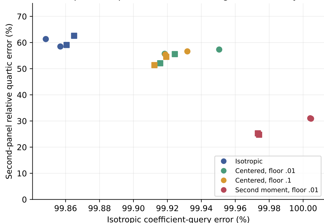
Empirical improvement trades off global accuracy
