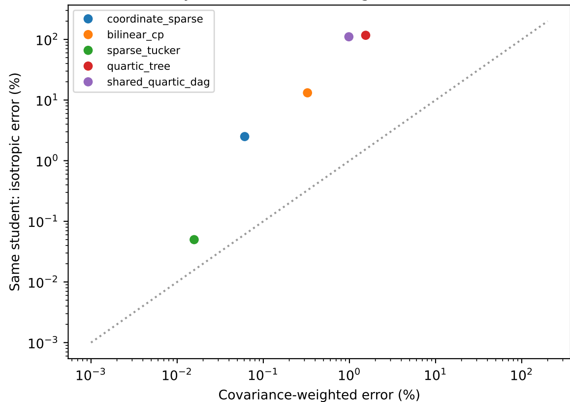
Toy covariance: best weighted-loss fits
