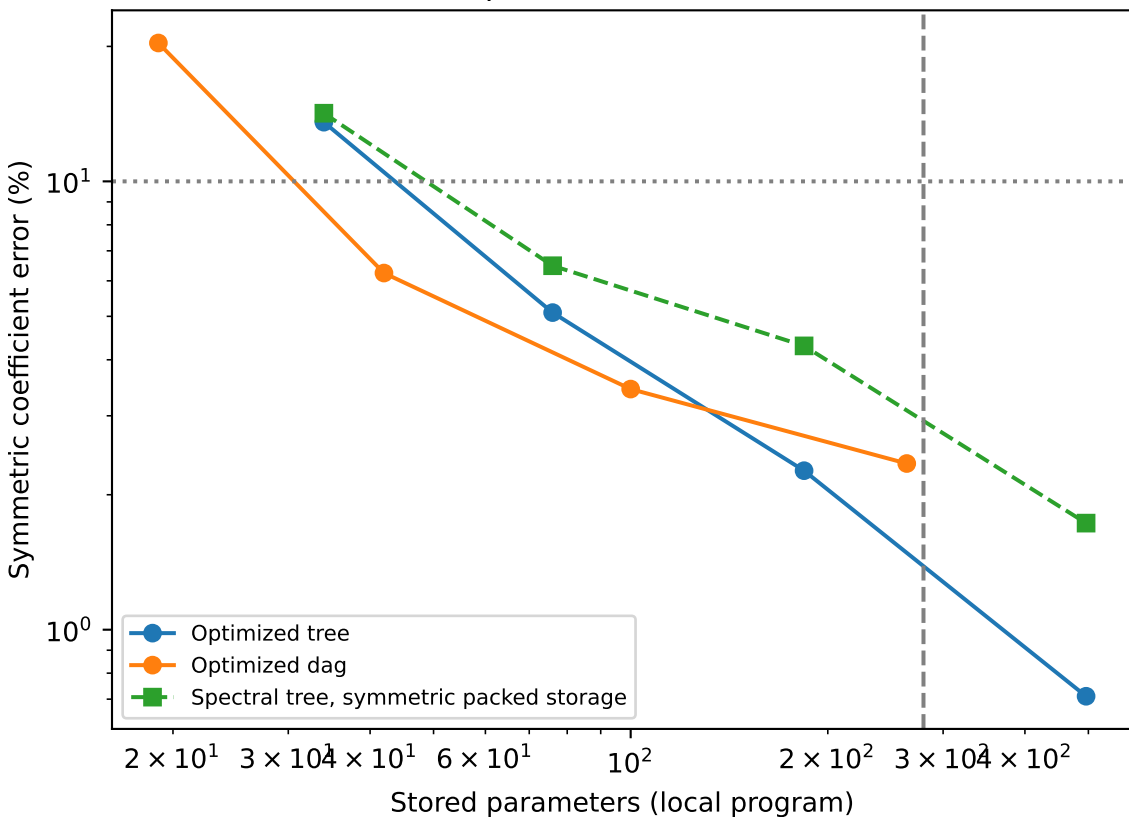
Native quartic: one fixed context
