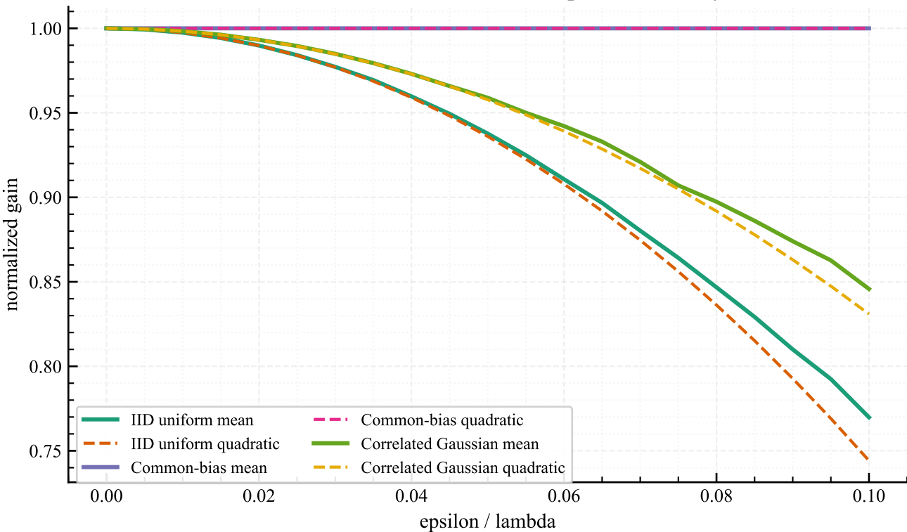
Cross-scenario validation of the quadratic theory
