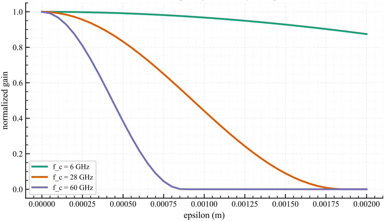
Carrier-frequency sensitivity sweep
