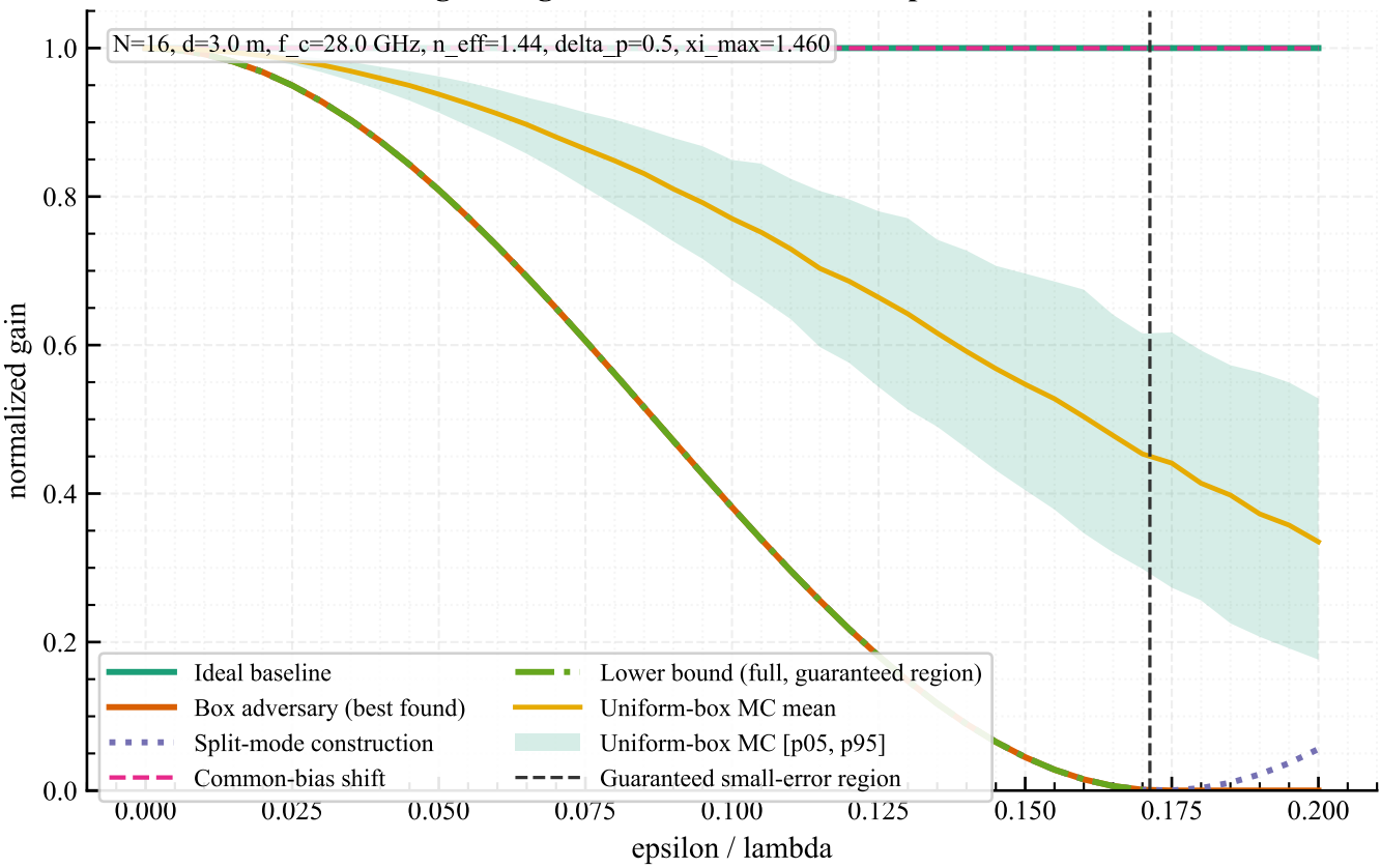
PASS gain degradation under bounded position errors
