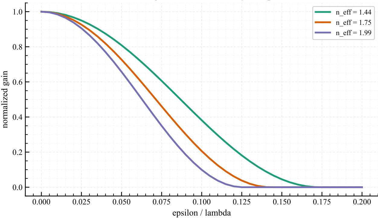
Waveguide-index sensitivity sweep
