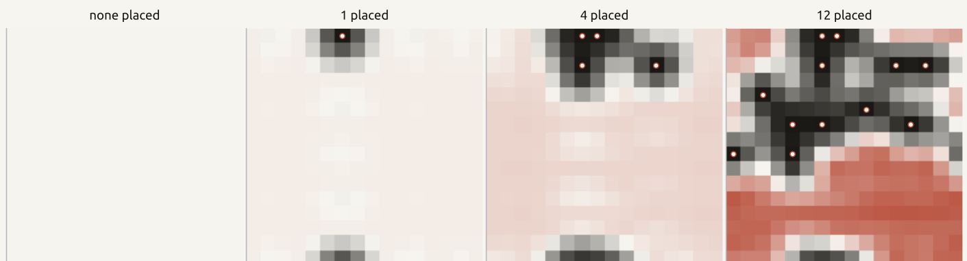
FIGURE 2 The exclusion hole. The chance that the next crystal lands on each site of a 16 x 16 Pauli tile, against the average site, with none of a golden roll's crystals placed, then 1, 4 and 12. Each placed crystal digs a dark hole around itself; an average site is pale, and the chance piles up, in the accent, where no crystal has yet landed. The tile wraps at its edges. The stock's own kernel, conditioned on golden roll 1, computed in float64 for the figure.
