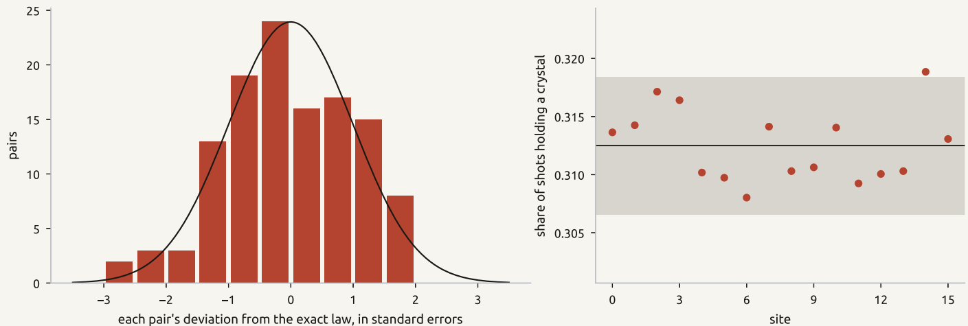
FIGURE 4 Atlas's 24,576 shots against the exact law. Left: for each of the 120 pairs of sites, how far the share of shots with crystals on both sat from the law's chance, in standard errors; the curve is what chance alone would give. Right: each site's share of shots holding a crystal, against the law's 5/16 and its band of two standard errors. Pooled through the decode rule from the committed results while this paper was built.
