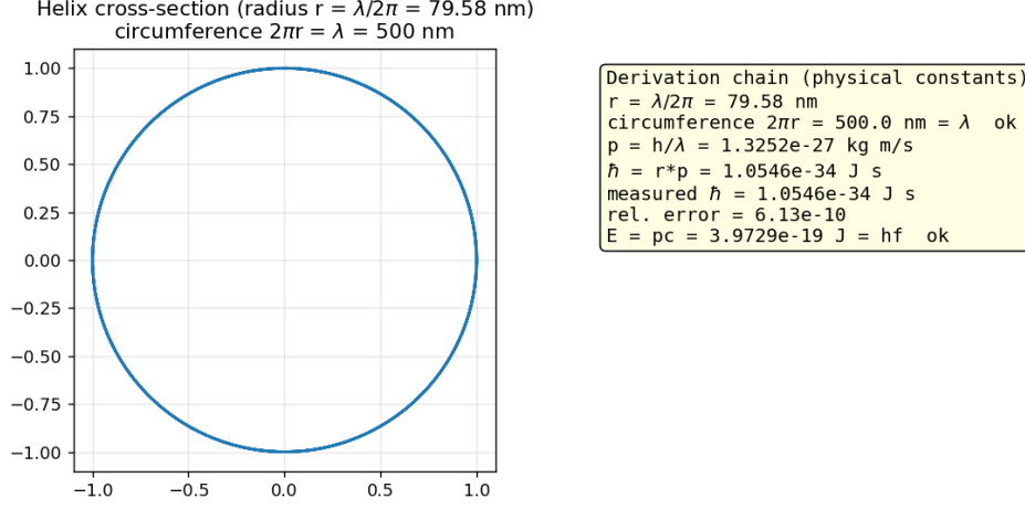
FIG. 6. Circumference = wavelength: the helix cross-section has radius r = \lambda/2\pi (reduced wavelength); the circumference 2\pi r = \lambda . The derivation chain r = \lambda/2\pi \Rightarrow \hbar = rp \Rightarrow p = h/\lambda \Rightarrow E = hf is closed.
