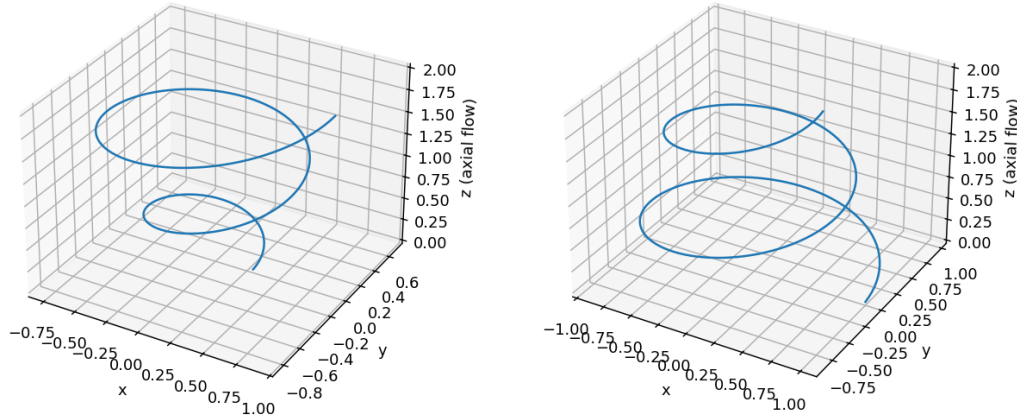
Positive charge: diverging right-handed helix (source) Negative charge: converging right-handed helix (sink)
