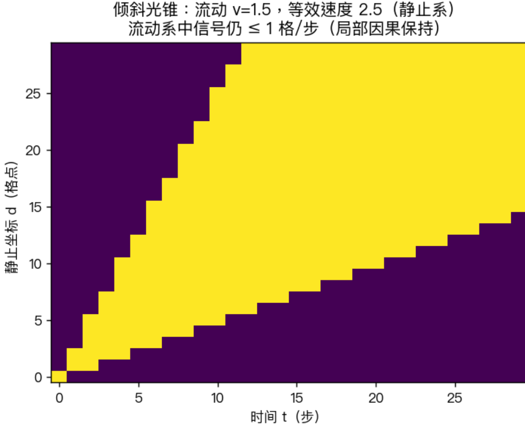
FIG. 2. Tilted light cone: with flow v = 1.5 the causal region in the rest frame has slope 1 + v (equivalent speed > 1 ), while in the flow frame signals remain \leq 1 per step.
