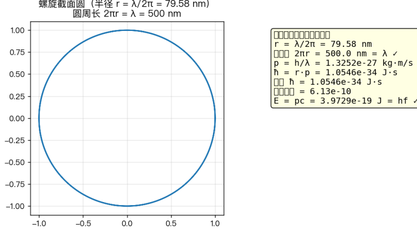
FIG. 6. Circumference = wavelength: the helix cross-section has radius r = \lambda/2\pi (reduced wavelength); the circumference 2\pi r = \lambda . The derivation chain r = \lambda/2\pi \Rightarrow \hbar = rp \Rightarrow p = h/\lambda \Rightarrow E = hf is closed.
