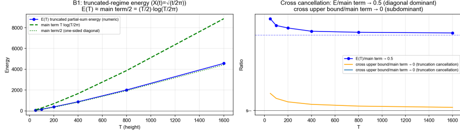
FIGURE 4. A numerical energy budget for truncated sums. The plot illustrates the harmonic scale; it is not used as a substitute for a zero-counting theorem.
