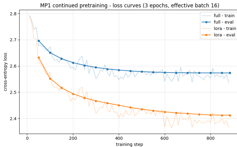
Figure 2: Training and validation loss for both runs (3 epochs, 12,000 training documents). Full fine-tuning in blue; LoRA in orange.
