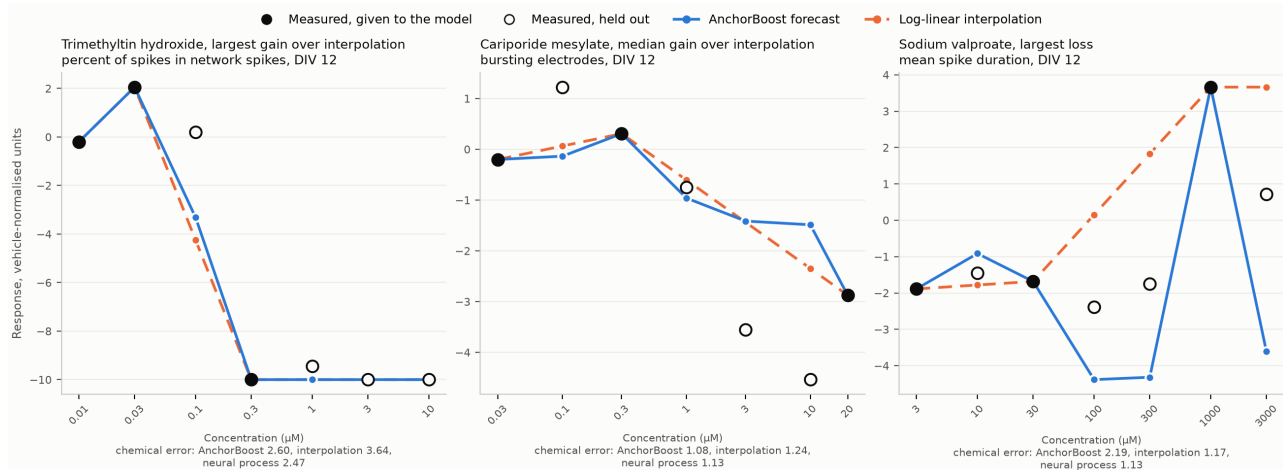
Figure 1: Measured and forecast DIV 12 responses for three held-out chemicals, each from its first published three-concentration design and its own fold model. Filled circles: concentrations given to the model; open circles: measured means held out; blue: AnchorBoost; dashed orange: log-linear interpolation. Each panel shows the feature whose measured means vary most across concentrations; chemical errors average all 68 outputs and five designs. Panels: the largest gain over interpolation, the median gain and the largest loss.
