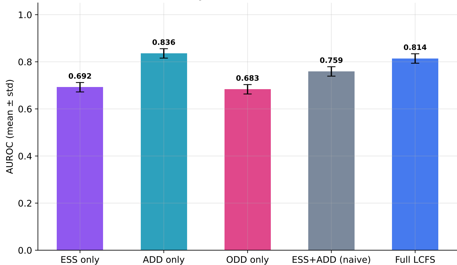
Ablation: Component Contribution to AUROC
