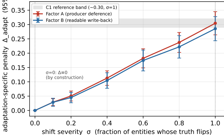
Severity-response of the structured-state feedback effect (controlled synthetic; 50 seeds; descriptive)
