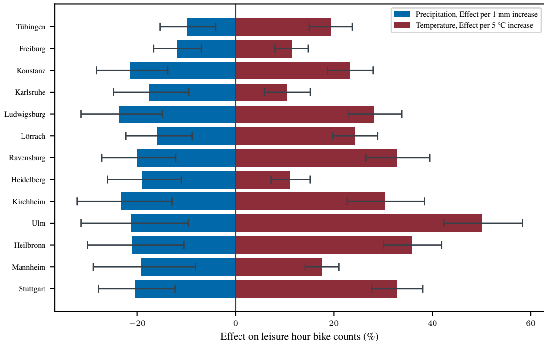
Precipitation and Temperature Effects by City
