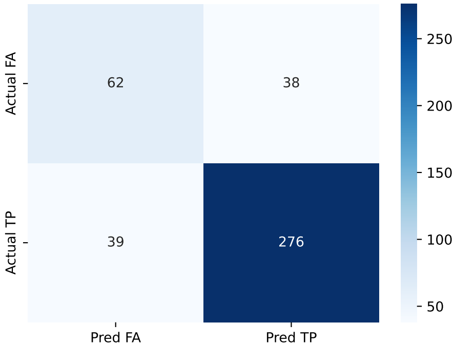
RQ3 — Confusion Matrix (XGBoost, best seed)
