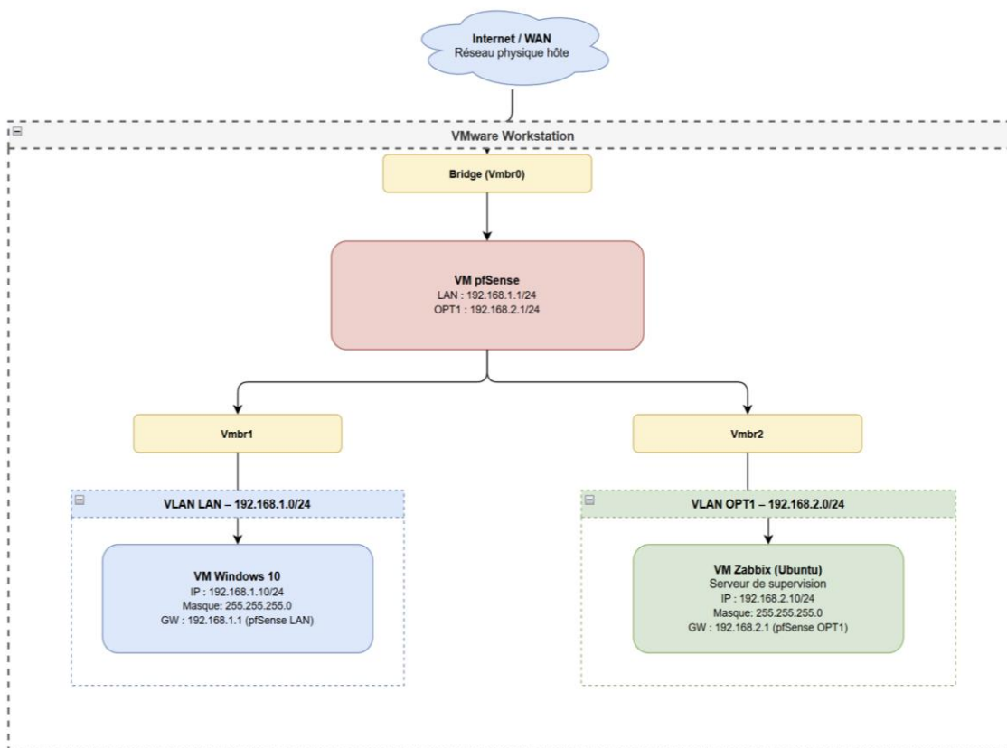
Architecture E6 – VMware Workstation
