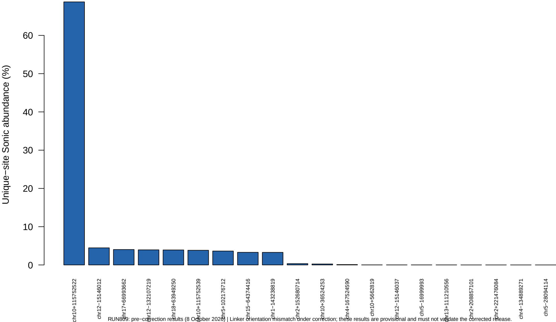
Top 20 insertion sites
