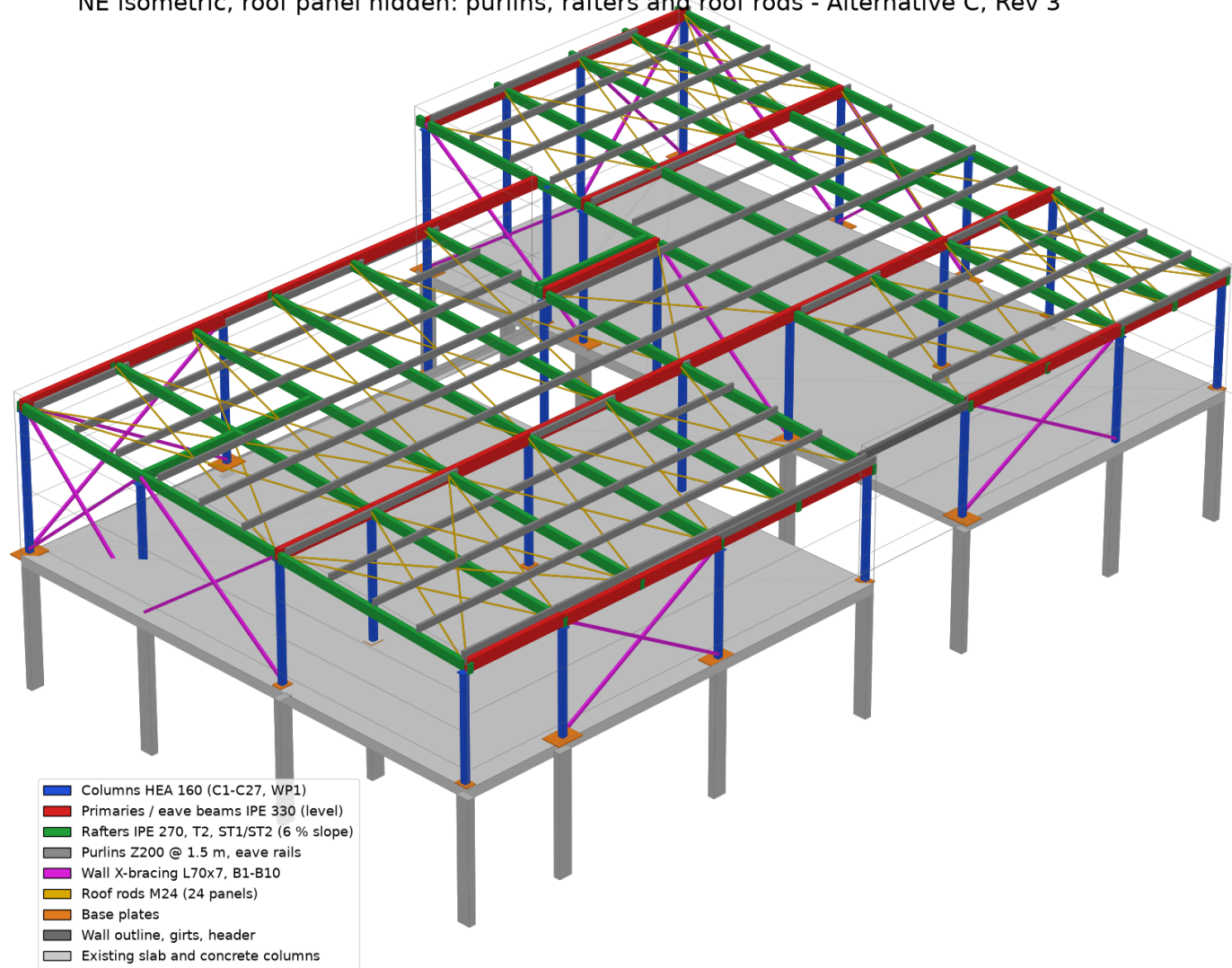
NE isometric, roof panel hidden: purlins, rafters and roof rods - Alternative C, Rev 3
