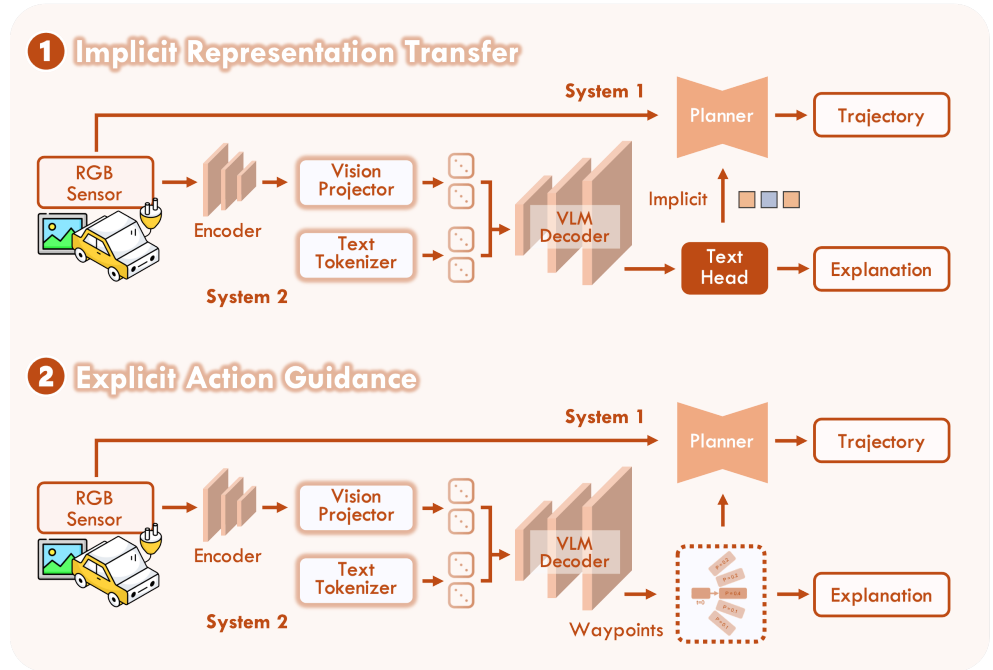
Figure 6: Dual-System VLA
