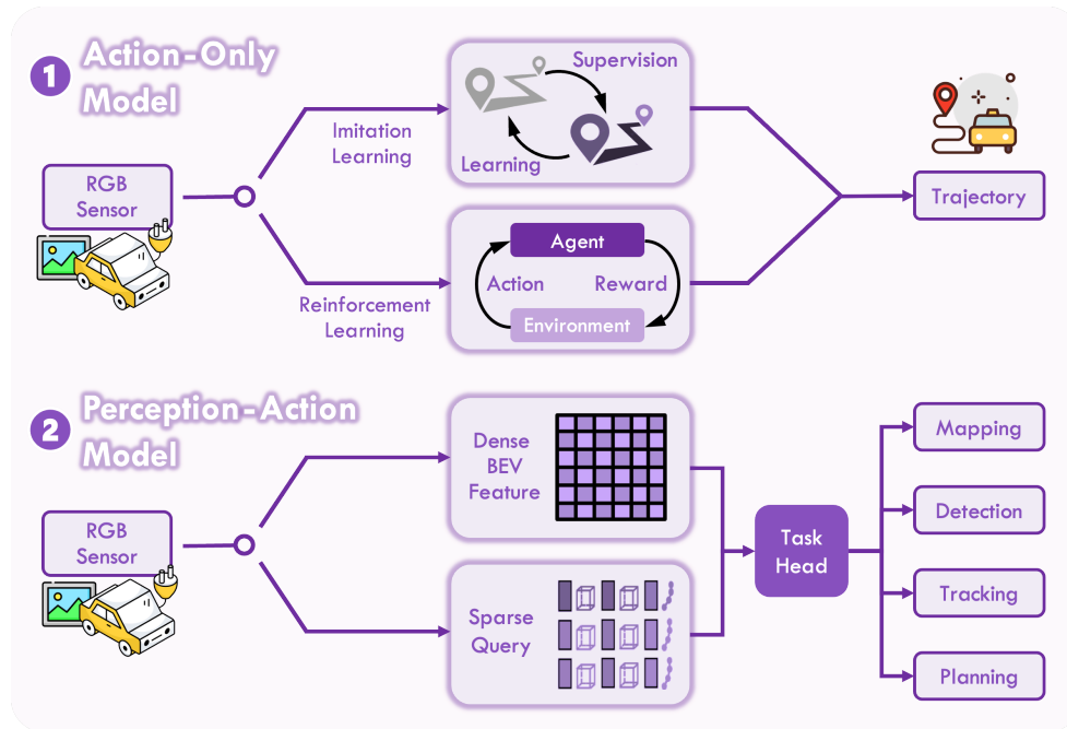
Figure 3: End-to-End Models
