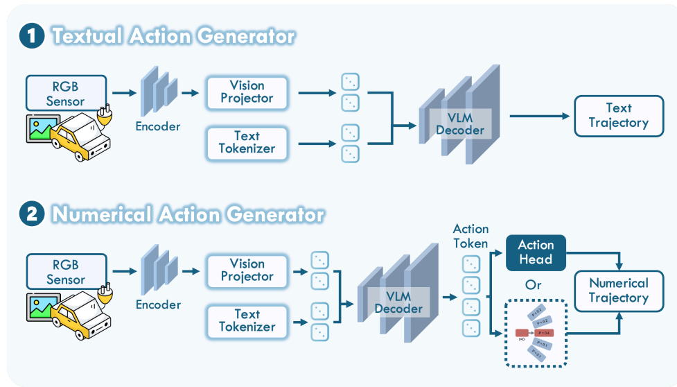
Figure 5: End-to-End VLA
