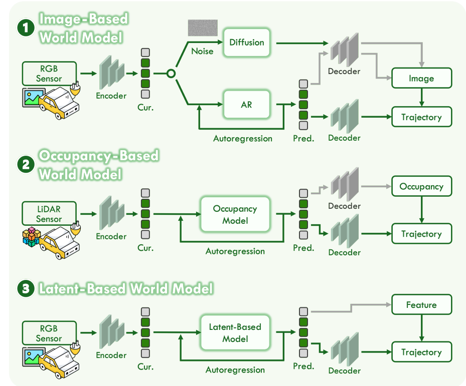
Figure 4: World Models
