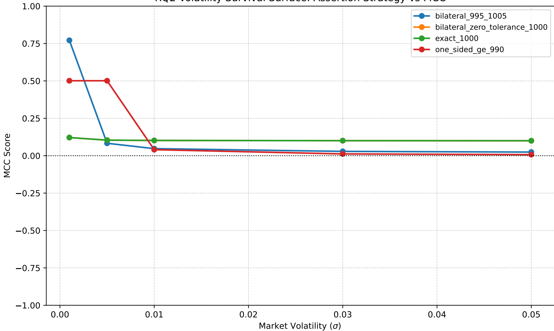
RQ2 Volatility Survival Surface: Assertion Strategy vs MCC
