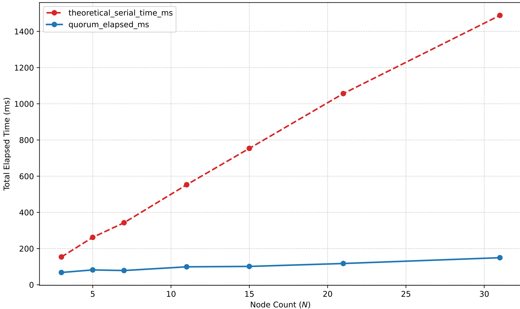
RQ3 Async Scaling Advantage
