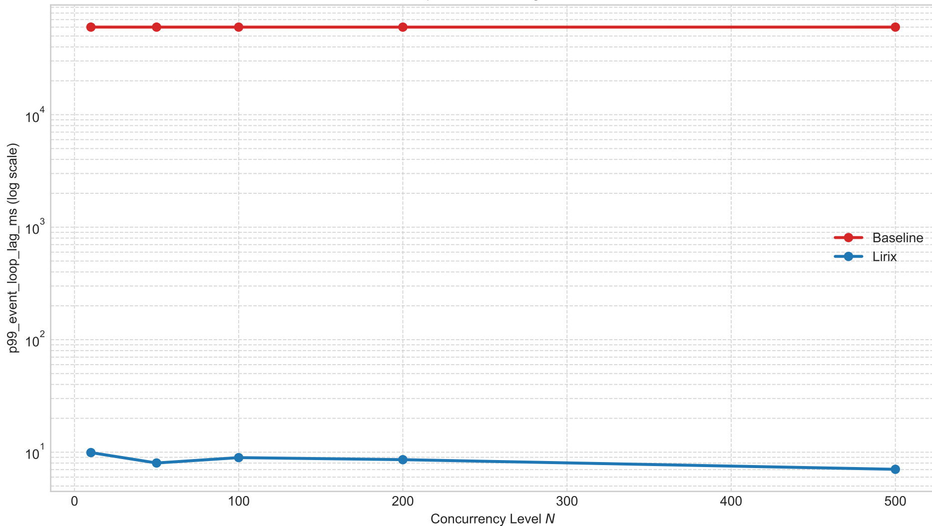
RQ1 Event-loop Heartbeat Lag: Baseline vs Lirix
