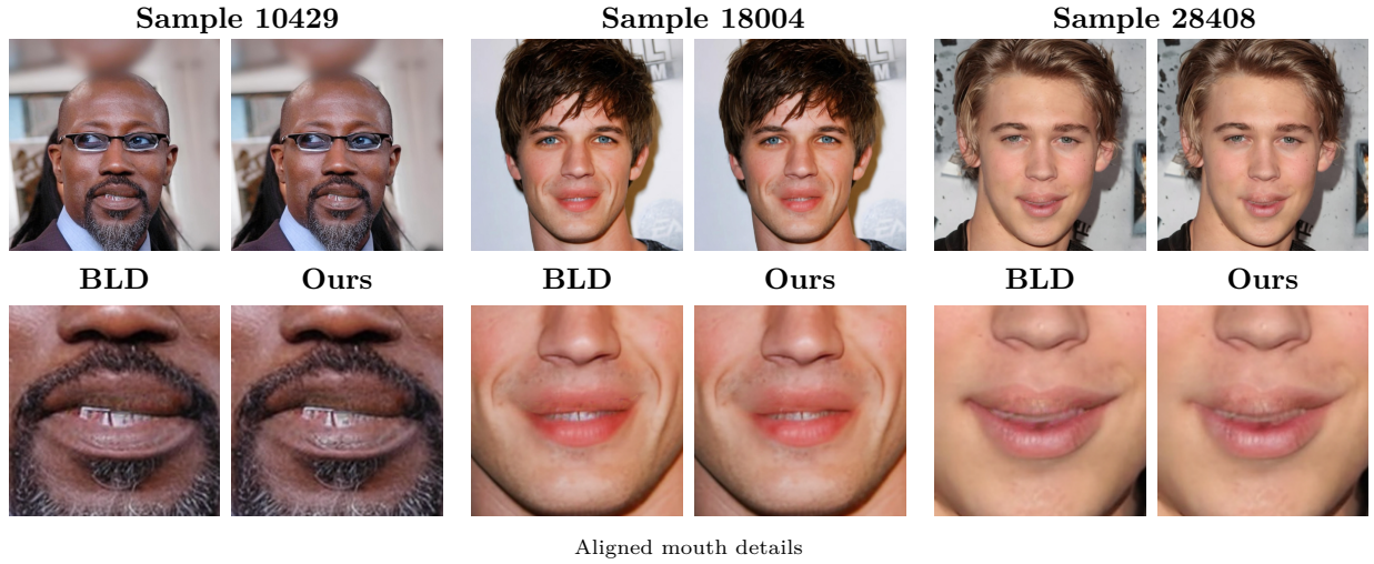
Figure 2: Paired qualitative comparison. Within each pair, raw BLD and adaptive CCI share the source, semantic mask, prompt, seed, scheduler, localized attack, and generation settings. Full faces are shown so the localized mouth edit can be judged together with identity and background preservation; aligned mouth details expose the target evidence at print scale. Images are unretouched evaluation artifacts apart from resizing and cropping.
