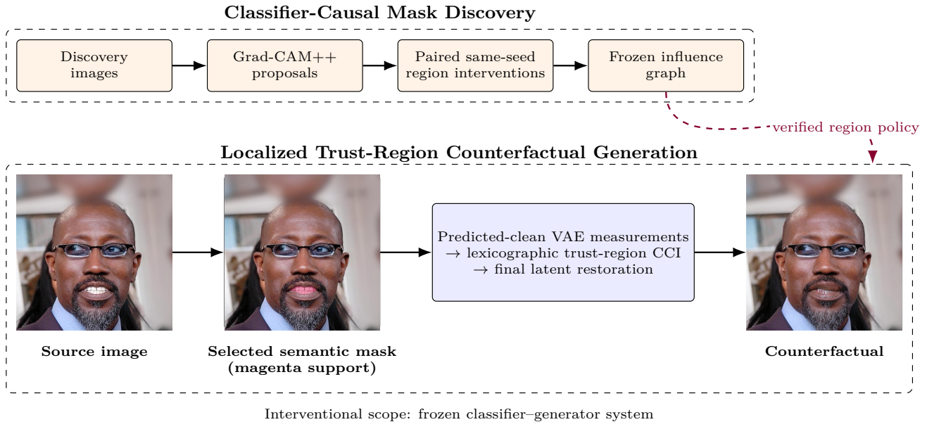
Figure 1: End-to-end method overview. The offline discovery stage turns saliency proposals into a verified classifier-specific influence graph. For a new source, the frozen policy determines the semantic intervention mask; predicted-clean lexicographic guidance and final latent restoration then produce one localized counterfactual. The real image panels are unretouched evaluation artifacts apart from resizing and the magenta mask overlay. Causal claims are limited to the frozen classifier-generator system.
