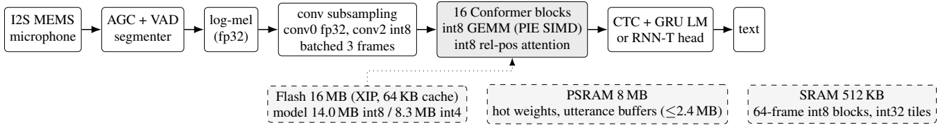
Figure 1: Oído on the ESP32-S3: pipeline and memory placement. Weights are streamed from flash or PSRAM once per 64-frame block. The activations of the current block and the int32 accumulation tiles stay in on-chip SRAM.
