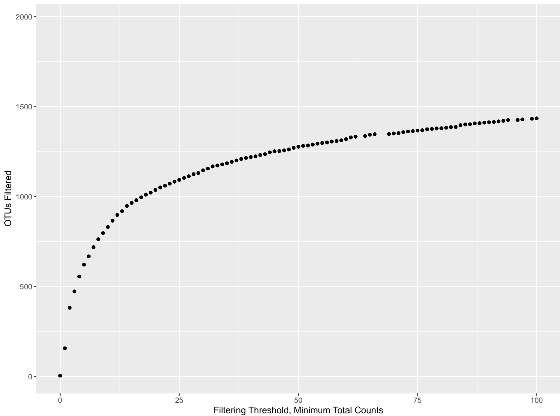
OTUs that would be filtered vs. the minimum count threshold
