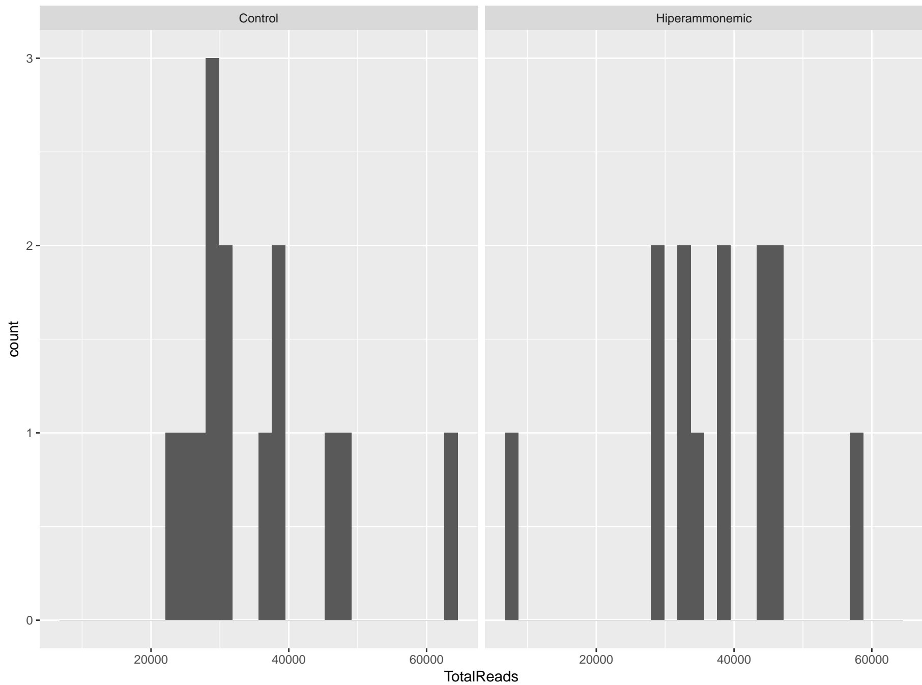
Sequencing Depth
