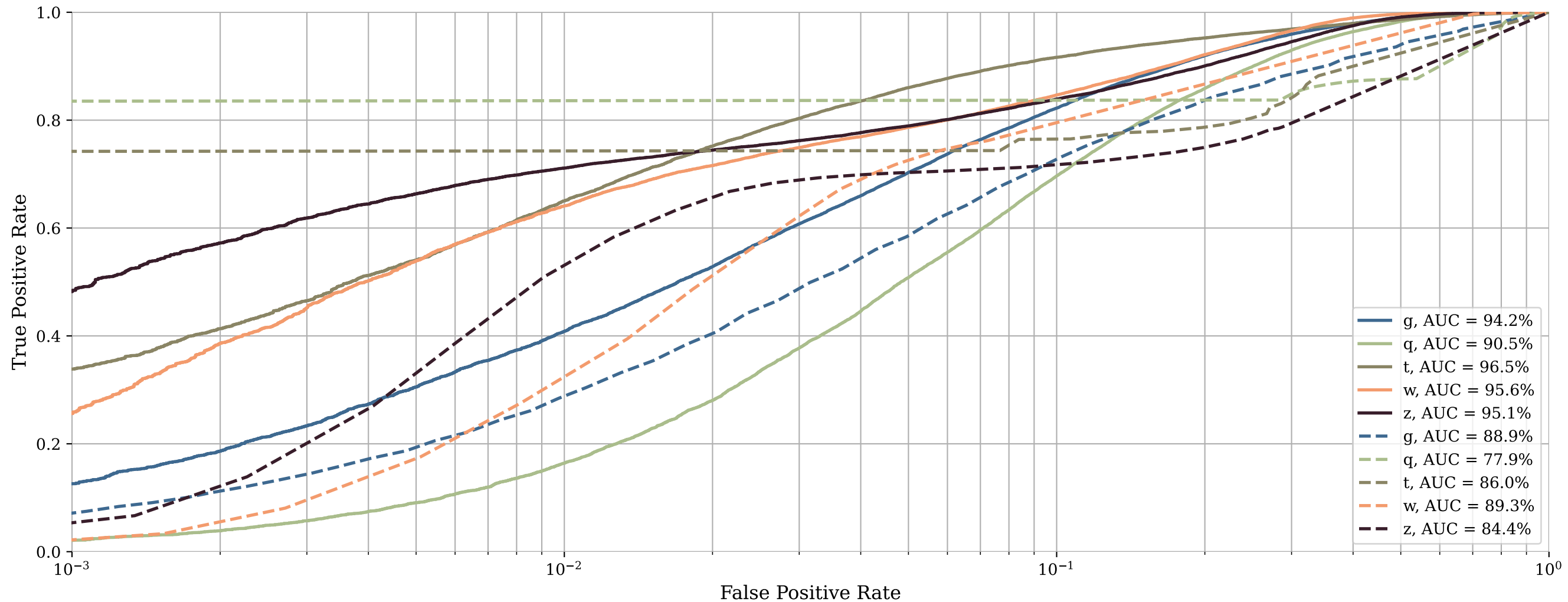
y_dut_Training_AdaptiveHP_acc=0.7117_ebops=303_VU_DA_bitfile.npy
