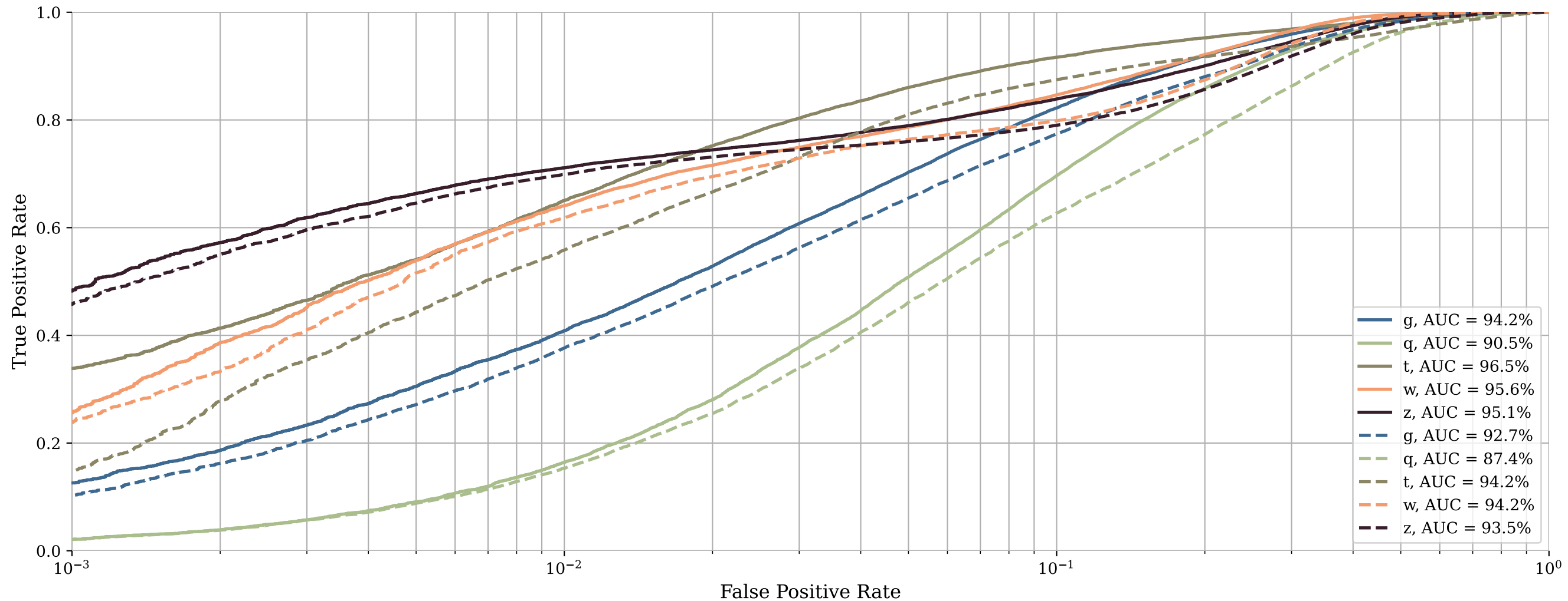
y_dut_Training_FixedHP_acc=0.7590_ebops=11634_VU_DA_bitfile.npy
