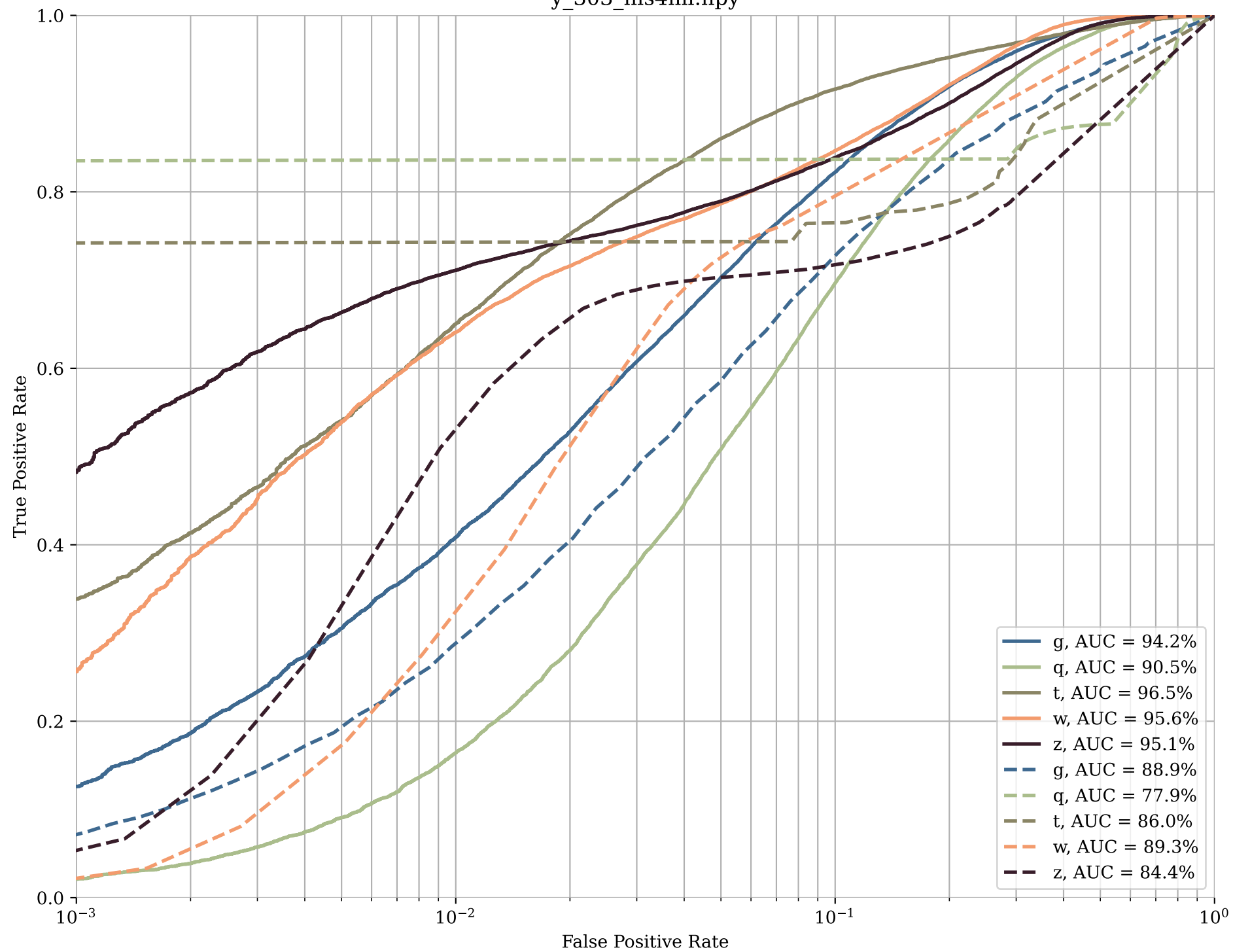
y_303_hls4ml.npy
