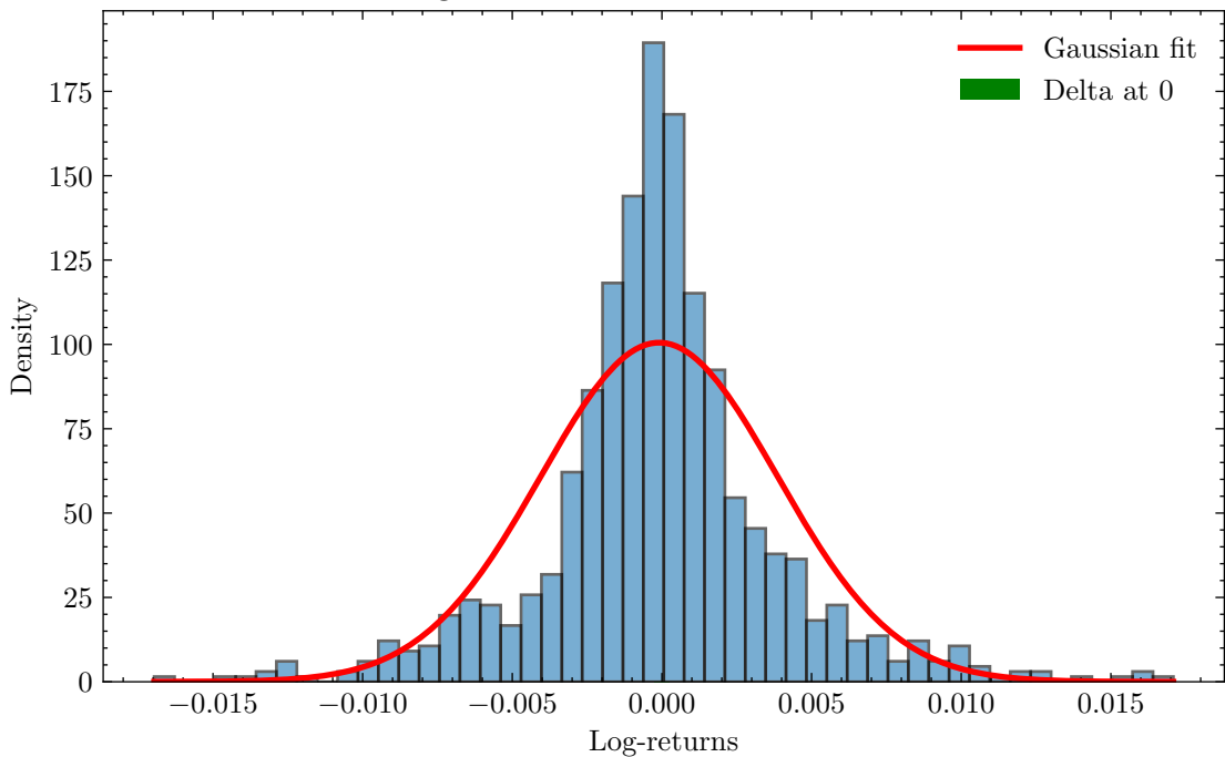
Histogram with Gaussian + Delta: EUR
