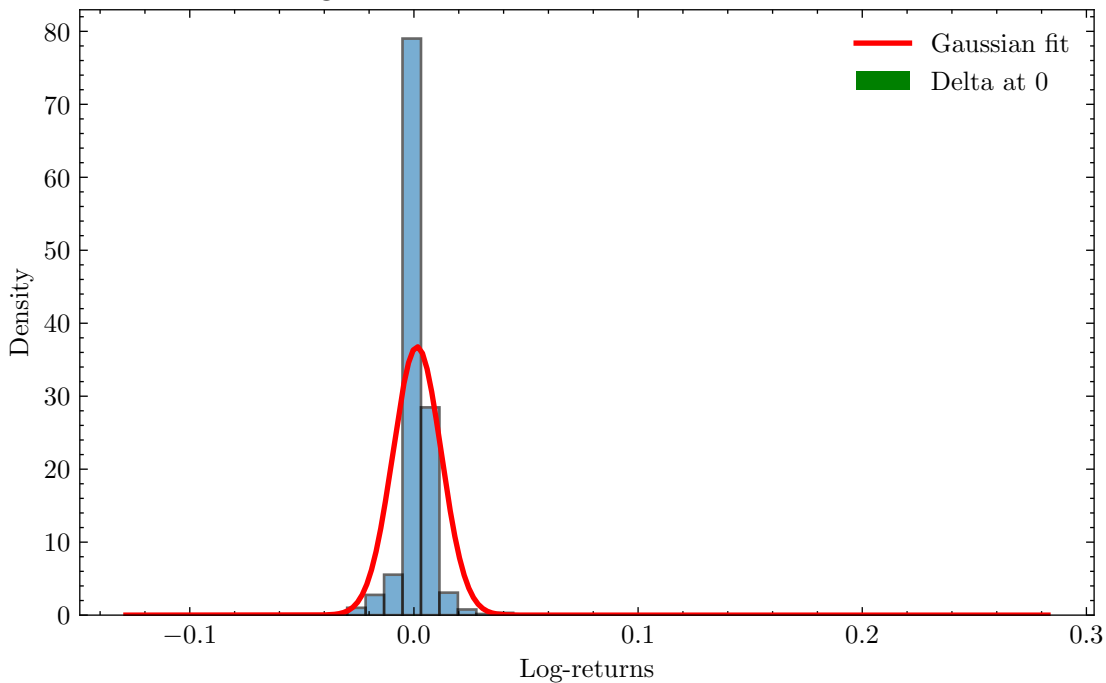
Histogram with Gaussian + Delta: USDCUP_Sell
