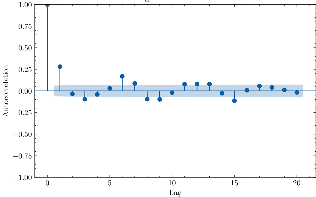
ACF of log-returns: blue_dollar_sell
