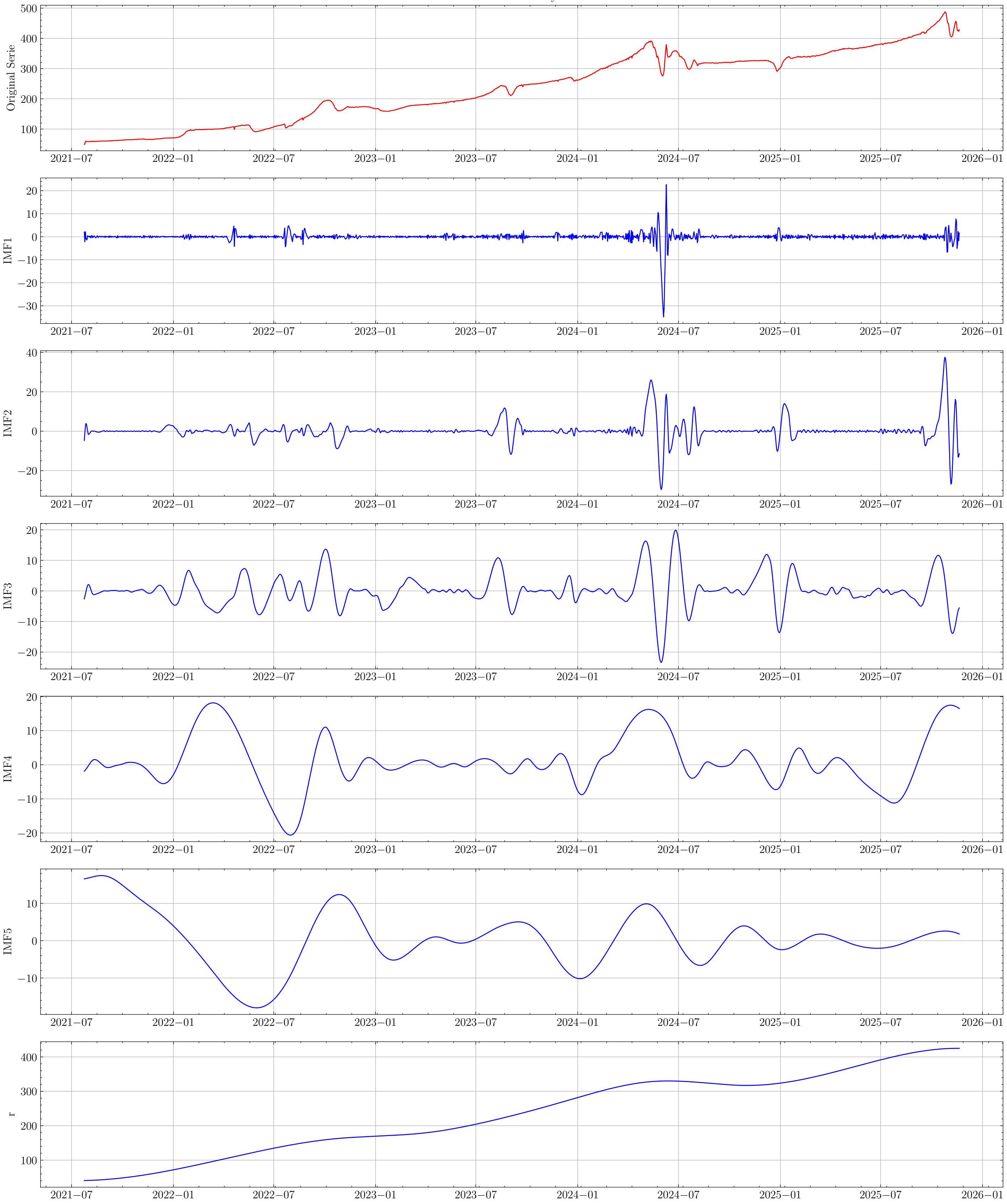
USDCUP_Buy
