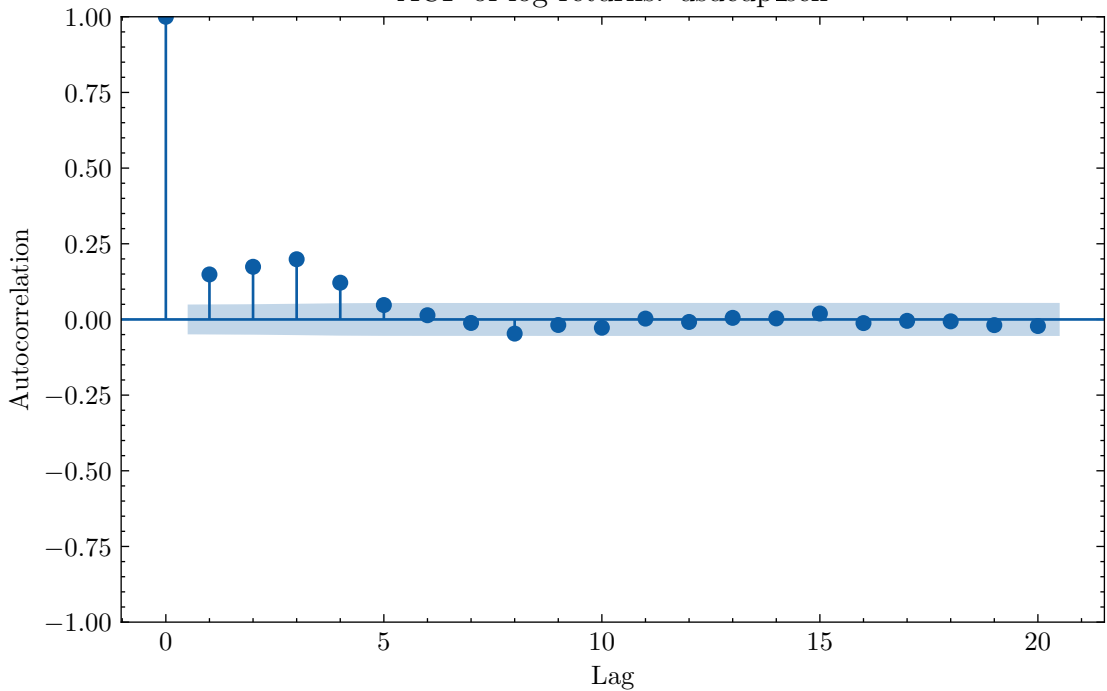
ACF of log-returns: usdcup_sell
